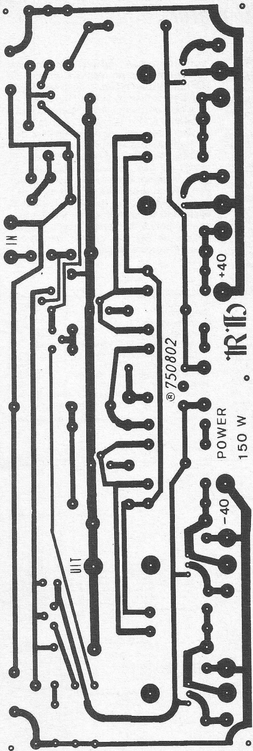
Fig. 4b Sporenplan
