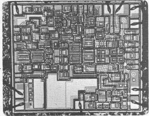
Sample and Hold Gated Operational Amplifier.
